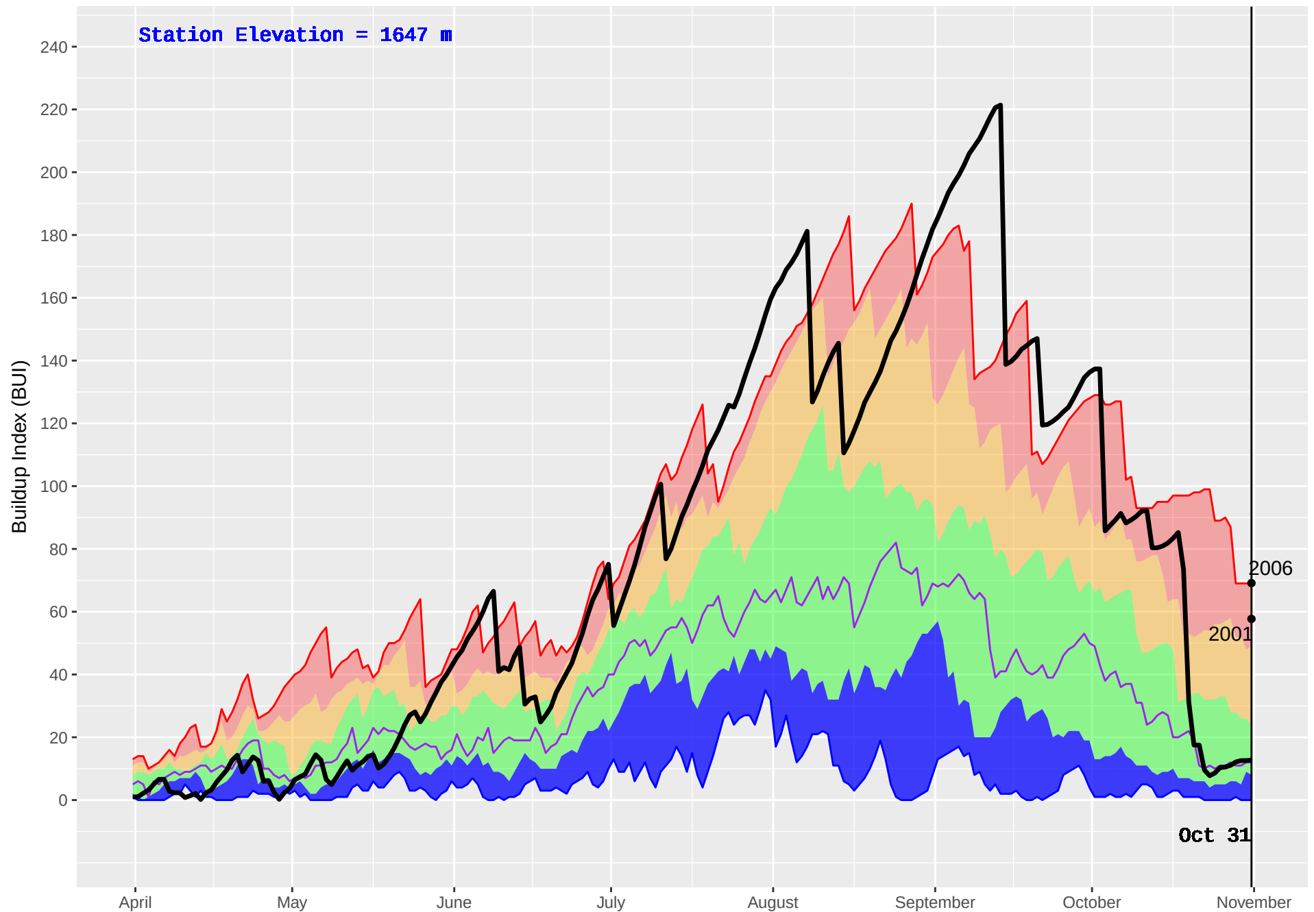
ROUND PRAIRIE (788) : Historical (2001–2016) and Current (2017) Noon Buildup Index (BUI)
